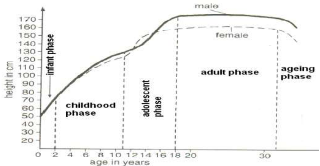
Fig 2.3: Growth Curve
