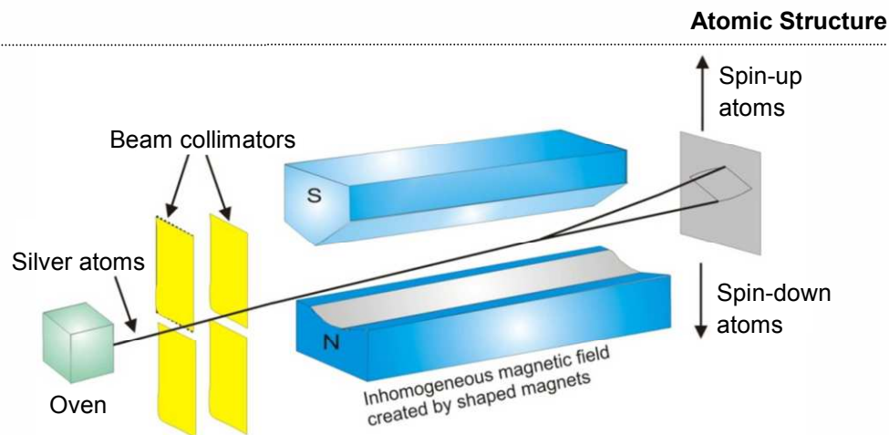
Fig. 4.15: Stern-Gerlach experiment.
