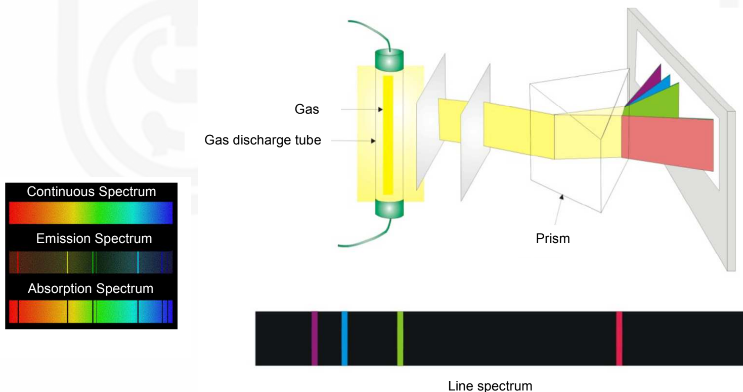
Fig.1.9: Line Spectrum.
