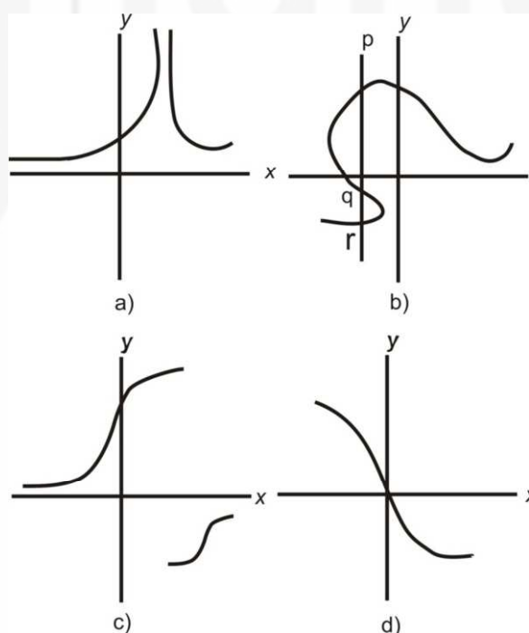
Fig. 3.1: Pictorial representation of wave functions; the curves a), b) and c) represent the functions which are not well behaved while d) shows the well behaved function.
