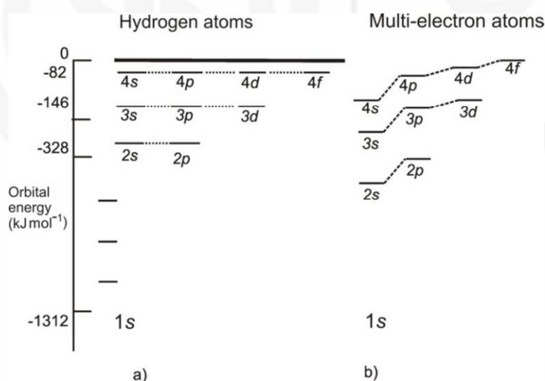
Fig. 5.1: a) Degenerate energy levels in case of hydrogen atom. b) Splitting of orbital degeneracy in multi-electron atoms.
