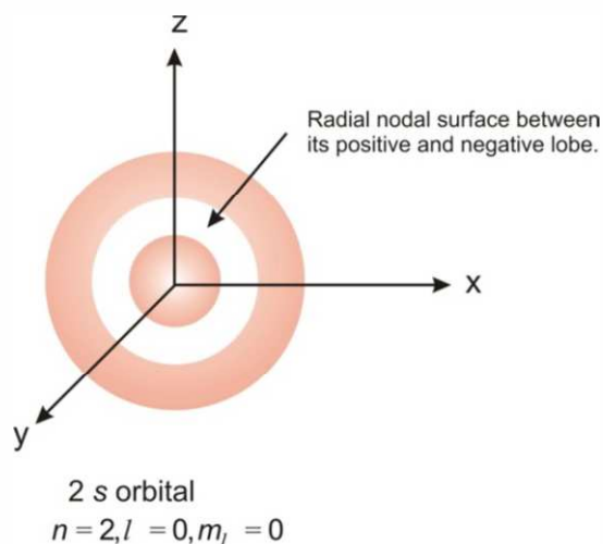
Fig. 4.10: Radial node in the 2s orbital.
