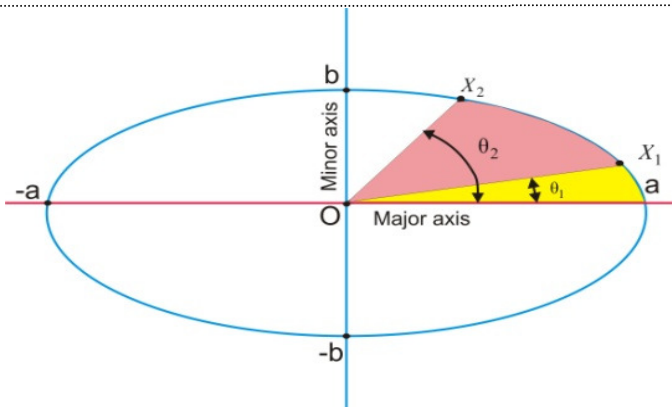
Fig. 1.13: Variation of the angle in an ellipse.
