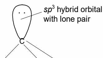
Trigonal pyramidal geometry of carbanion
