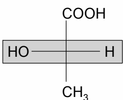
L-(+)-lactic acid
