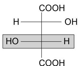
L-(–)-tartaric acid
