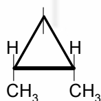
cis -1,2-dimethylcyclopropane
