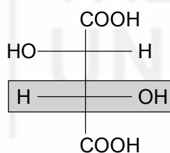
D-(–)-tartaric acid
