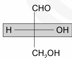
D-(+)-glyceraldehyde
