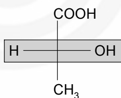
D-(–)-lactic acid
