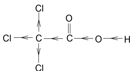
trichloroethanoic acid
