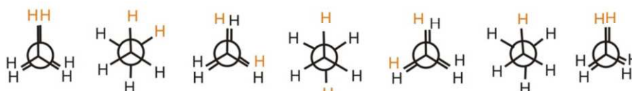
Fig. 12.3: Variation of potential energy with dihedral angle. Here, to make it easy to visualise the dihedral angle, the two hydrogens on the two carbons are shown in the different colour.
