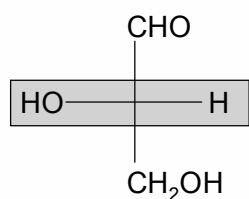
L-(–)-glyceraldehyde
