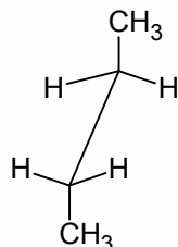
Sawhorse projection
