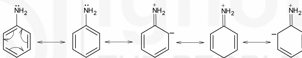
Resonance structures of aniline
