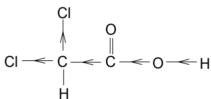
dichloroethanoic acid
