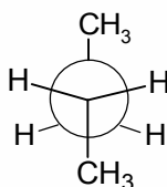
Newman projection
