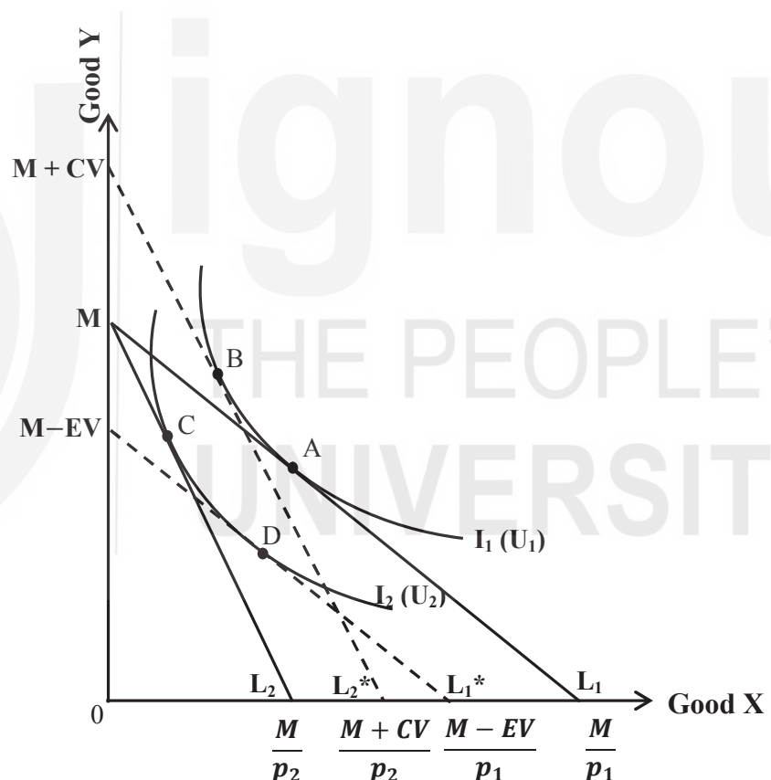
Fig. 3.10: Compensation and Equivalent variations
