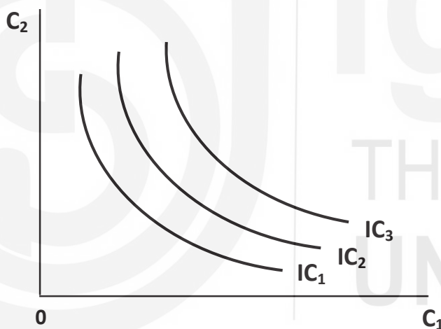
Fig. 4.8: Indifference Curves
