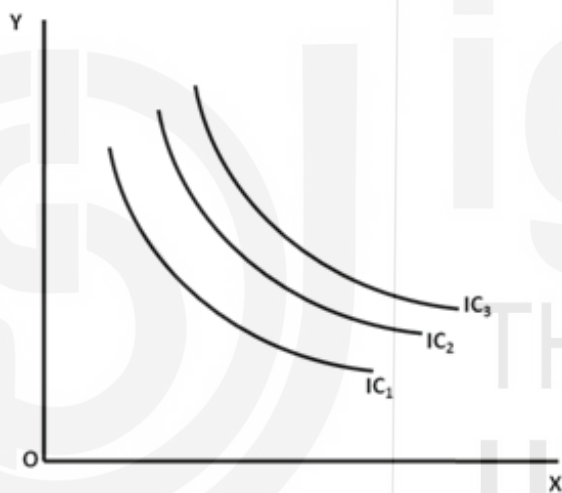
Fig. 1.3: Indifference Map
