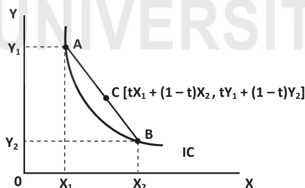
Fig. 1.4: Convex preferences
