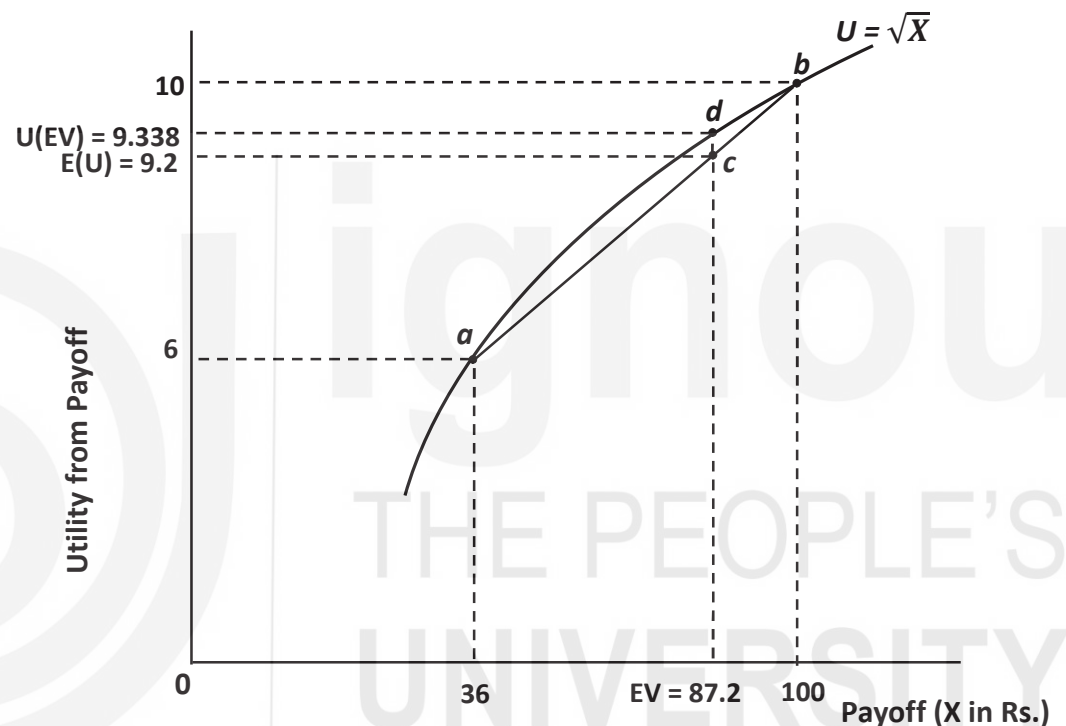
Fig. 4.4: Risk Aversion
