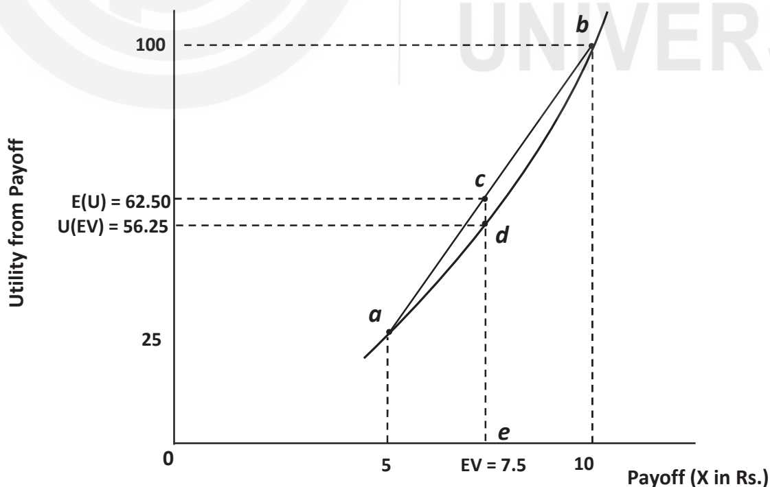
Fig. 4.5: Risk Preferring
