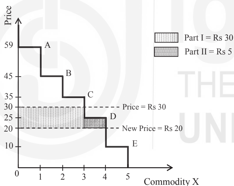
Fig. 3.6: Change in Consumer's Surplus resulting from a Price change for discrete good
