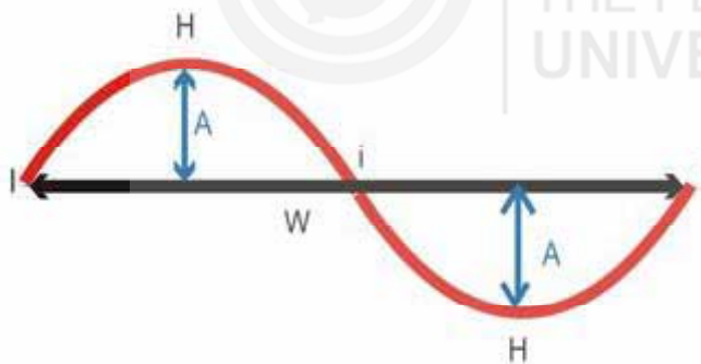
Fig. 10.1: Elements of fold (Abbreviations used: W-wavelength, A-amplitude, H-hinge point, i-inflexion point).
