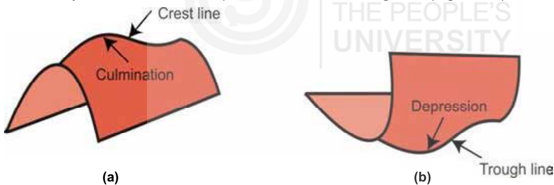
Fig. 10.4: a) Culmination; and b) Depression.
