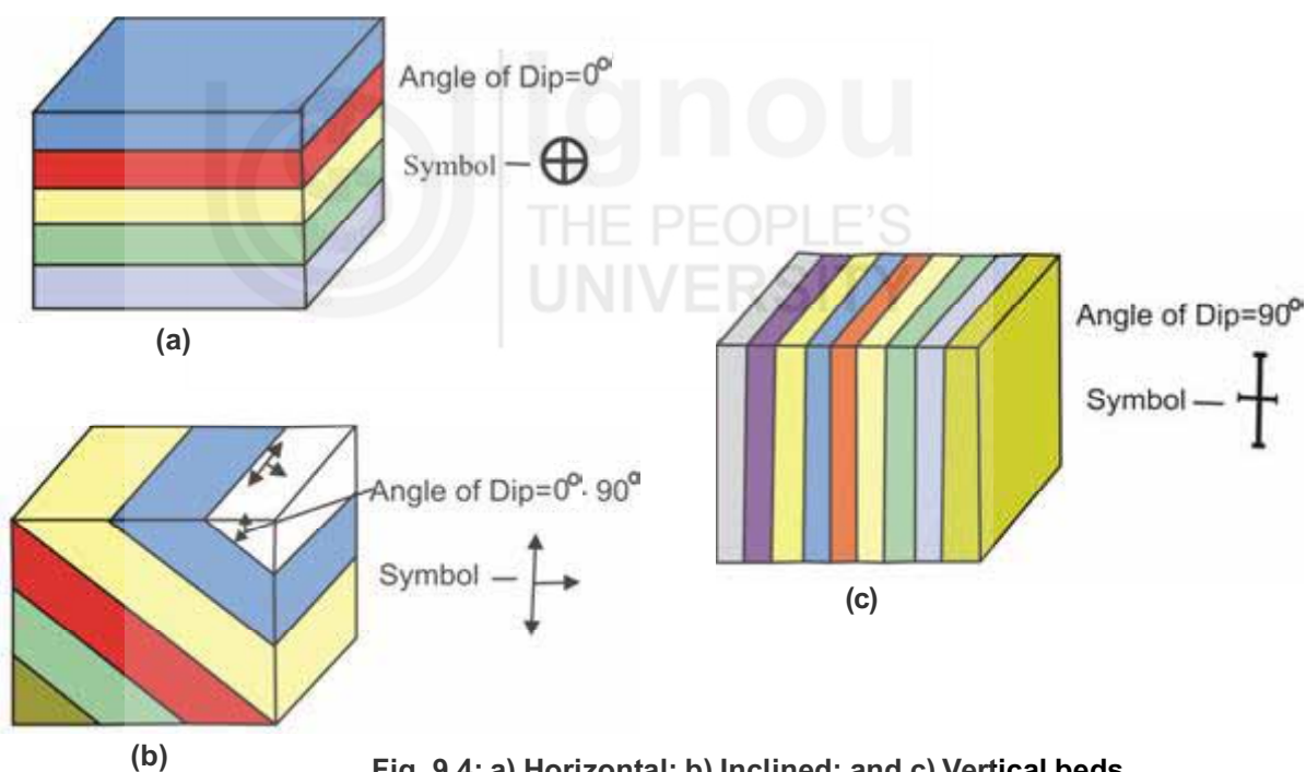
Fig. 9.4: a) Horizontal; b) Inclined; and c) Vertical beds.
