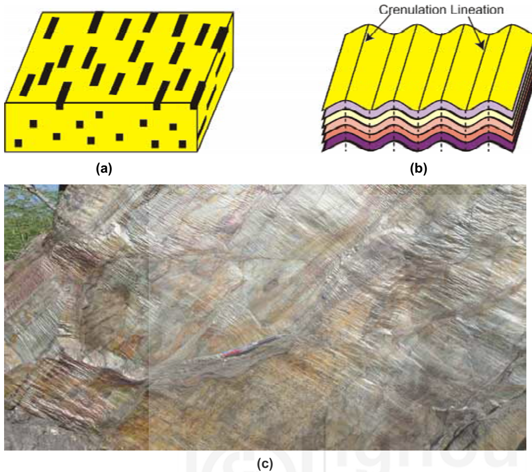
Fig.9.12: a) Mineral Lineation; b) Crenulation lineation; and c) Field photograph showing lineations. (Photo credit: Mr. Ganga Prasad Bhartiya)
