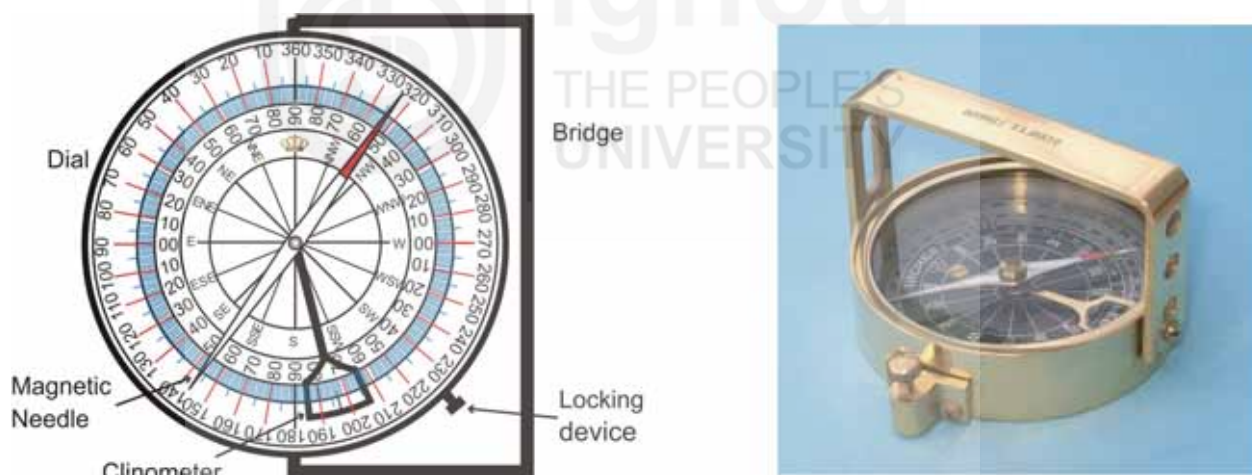
Fig. 9.14: Sketch and photograph of clinometer compass.
