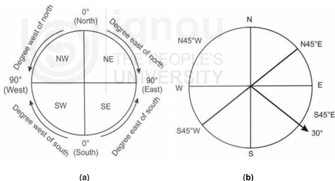
Fig. 13.13: Quadrant or bearing method of stating direction; (a) Four quadrants-NE, SE,SW,NW-are east or west of north or south and (b) Dip direction, strike direction and dip amount plotted in quadrant method
