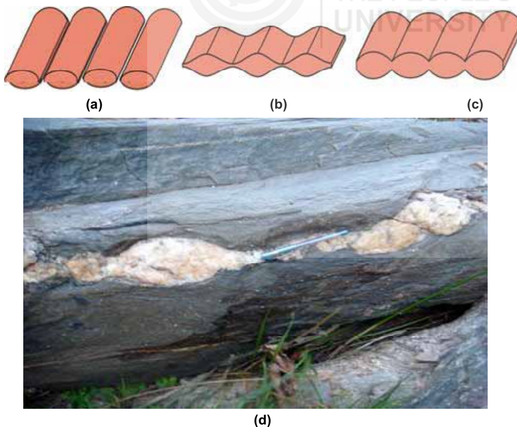
Fig. 9.13: a) Boudinage; b) Pinch and Swell structure; c) Mullion/Rodding structure; and d) Field photograph of pinch and swell structure. (Photo credit: Ganga Prasad Bhartiya)
