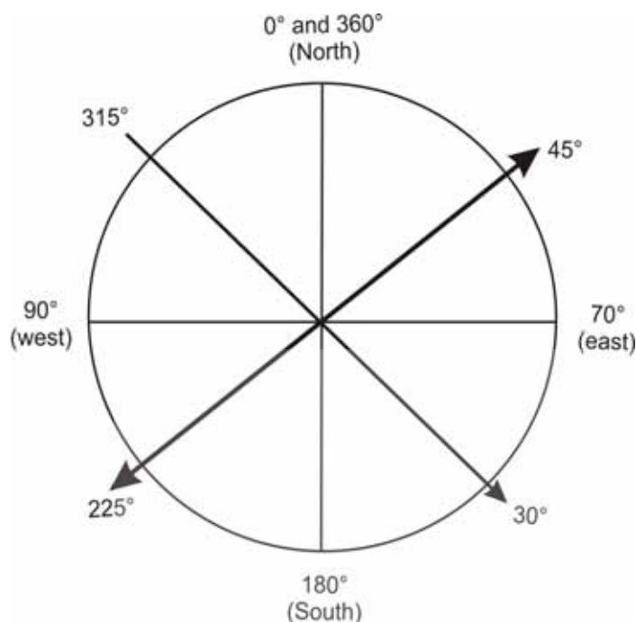
Fig. 13.14: The azimuth method of stating direction
