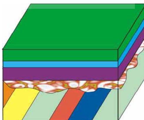
Fig. 12.10: Block diagram of an angular unconformity.
