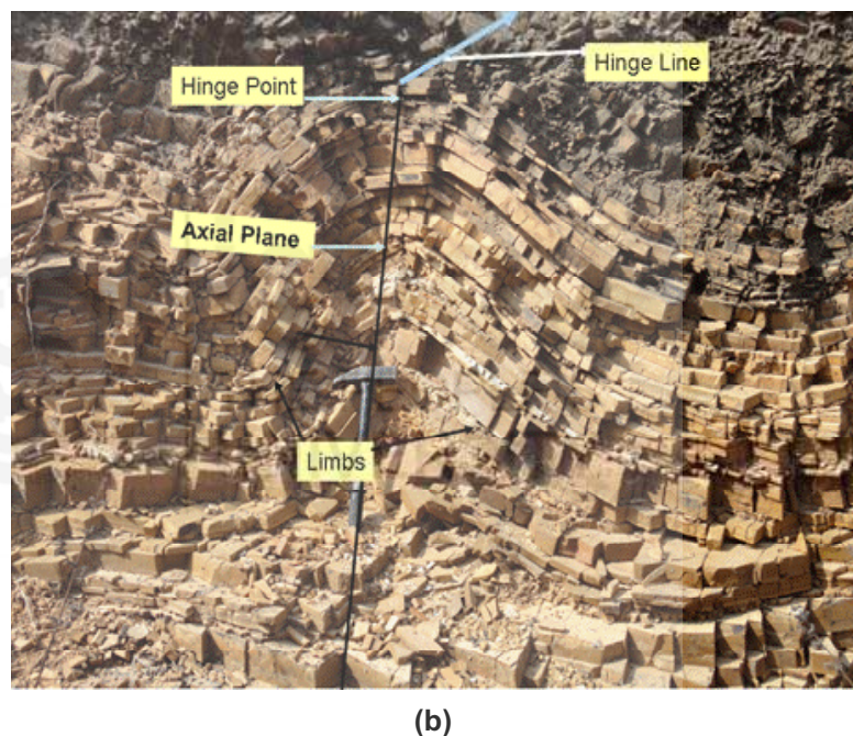
Fig. 10.2: a) Parts of a fold; and b) Field photograph of a fold.
