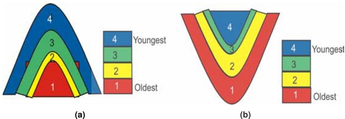
Fig. 10.8: a) Anticline/Antiformal anticline; and b) Syncline/Synformal syncline.
