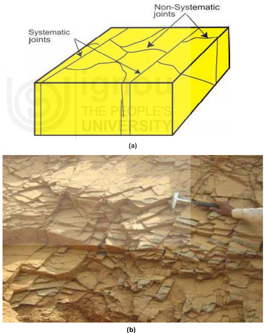
Fig. 12.1: Systematic and Non-systematic joints: a) Sketch; and b) Field photograph.
