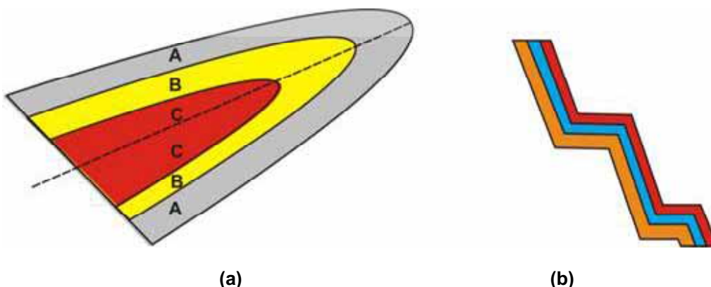
Fig. 10.21: a) Overtaken fold; and b) Structural Terrace.
