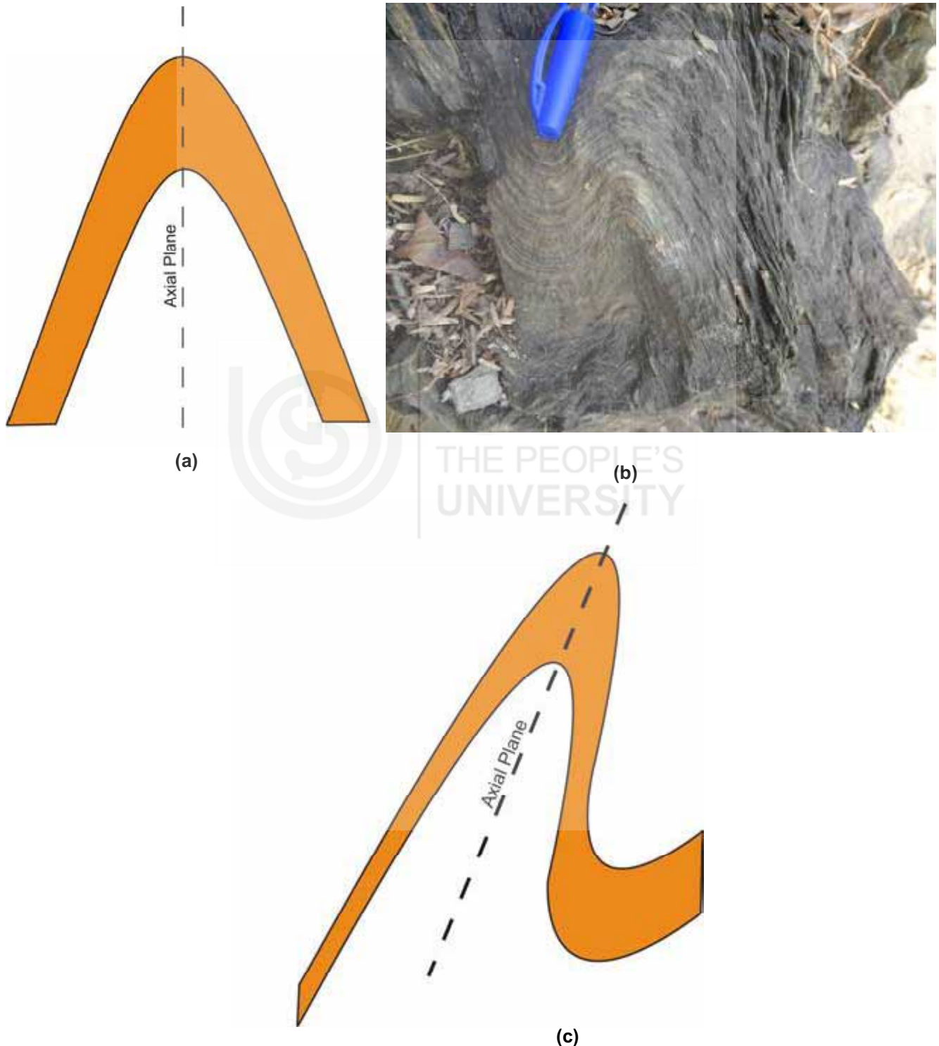
Fig. 10.11: a) Sketch of symmetrical fold; b) Field photograph of symmetrical fold in phyllite (Photo credit: Ganga Prasad Bhartiya); and c) Asymmetrical fold.
