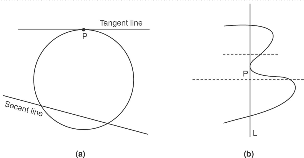
Fig. 4: Some curves and tangents to them
