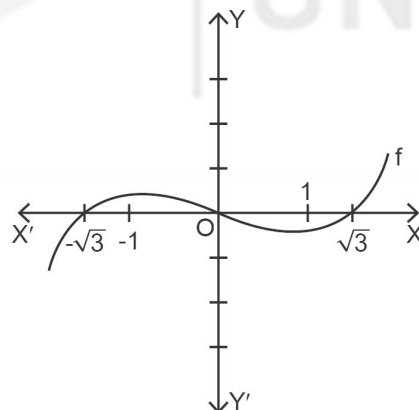
(a) Graph of f
