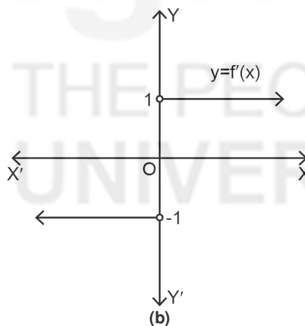
Fig. 12: Graphs of (a) f and (b) f'
