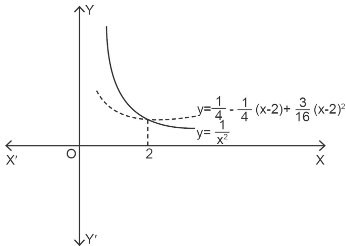
Fig. 8: Graph of f and p(x) about x = 2
