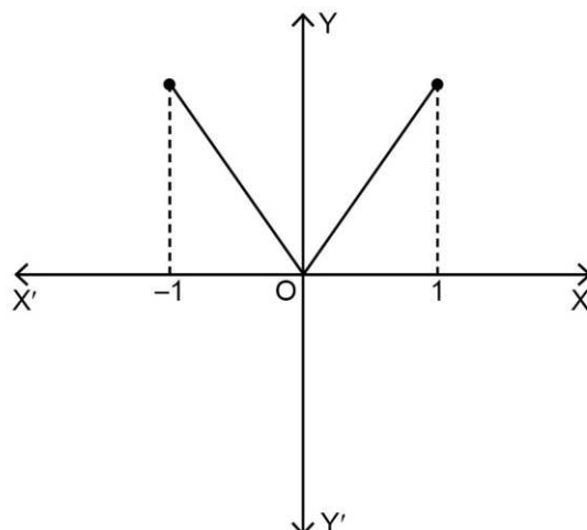
Fig. 29: Graph of f .
