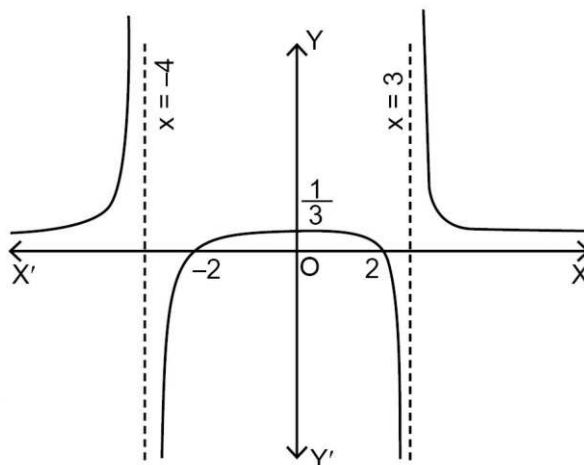
Fig. 4: Vertical asymptotes.
