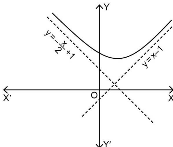
Fig. 16: Slant asymptotes.
