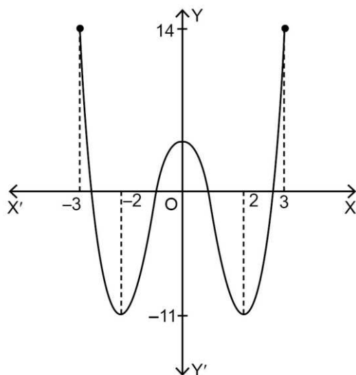
Fig. 13: Graph of f .
