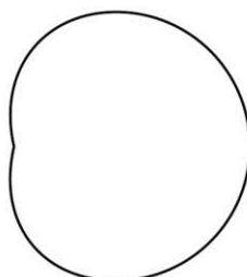
(g) 1 < \frac{a}{b} < 2 (Dimpled)
