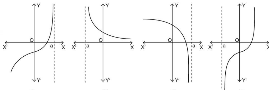
Fig. 5: Vertical Asymptotes.
