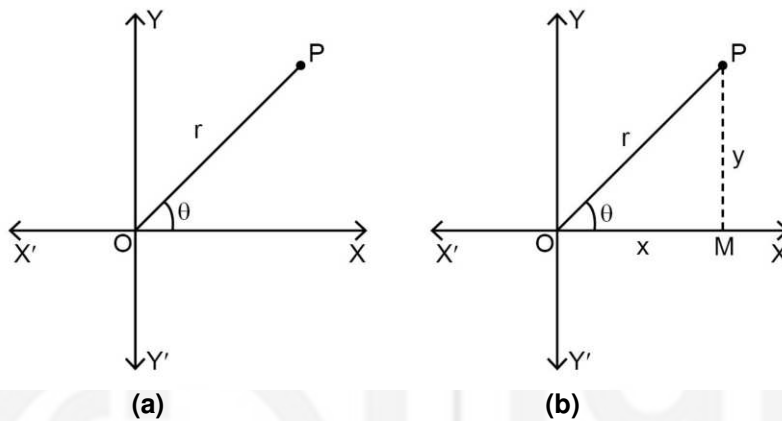
Fig. 30: Polar Coordinates.
