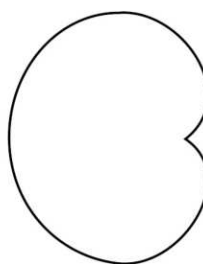
(b) r = a - b \cos \theta
