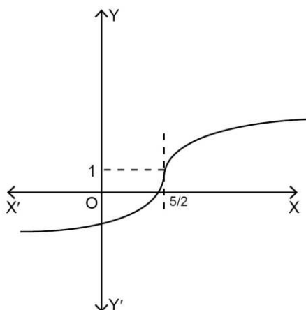
Fig. 12: Graph of y = (2x - 5)^{1/3} + 1 .
