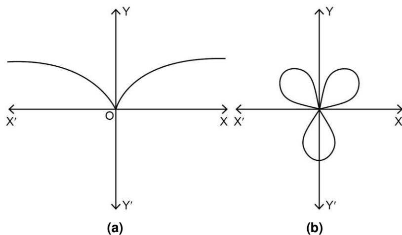
Fig. 34: Double and Multiple point.
