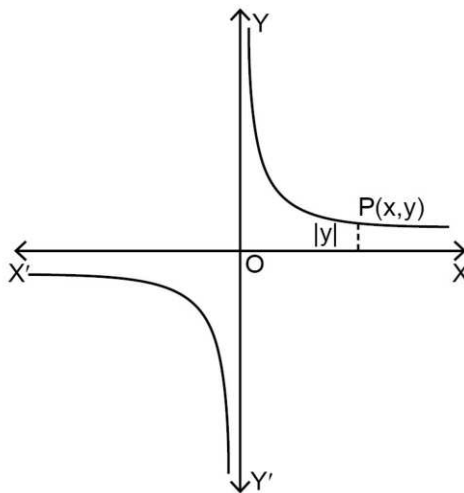
Fig. 1: Graph of xy = c .
