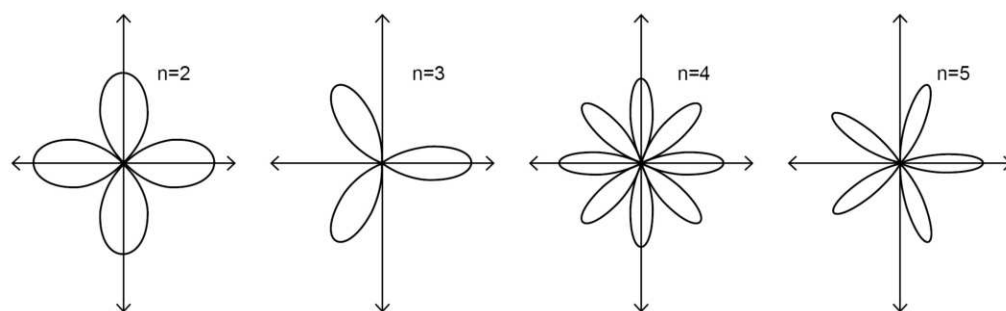
(b) r = a \cos n\theta .
