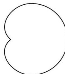
(f) \frac{a}{b} = 1 (Cardioid)
