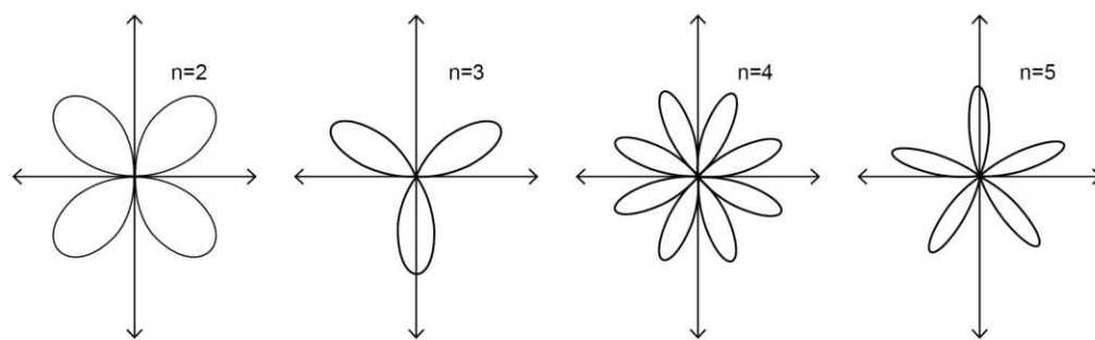
(a) r = a \sin n\theta .
