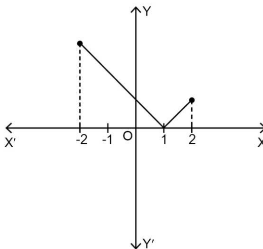
Fig. 6: Graph of f .
