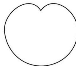
(c) r = a - b \sin \theta
