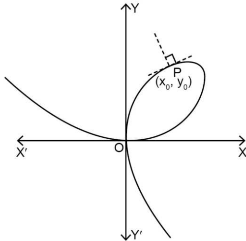
Fig. 24: Graph of x^3 + y^3 - 6xy = 0 .
