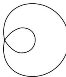
(e) \frac{a}{b} < 1 (with inner loop)
