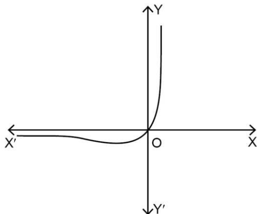
Fig. 12: Graph of y = x e^x .
