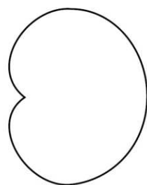
(a) r = a + b \cos \theta
