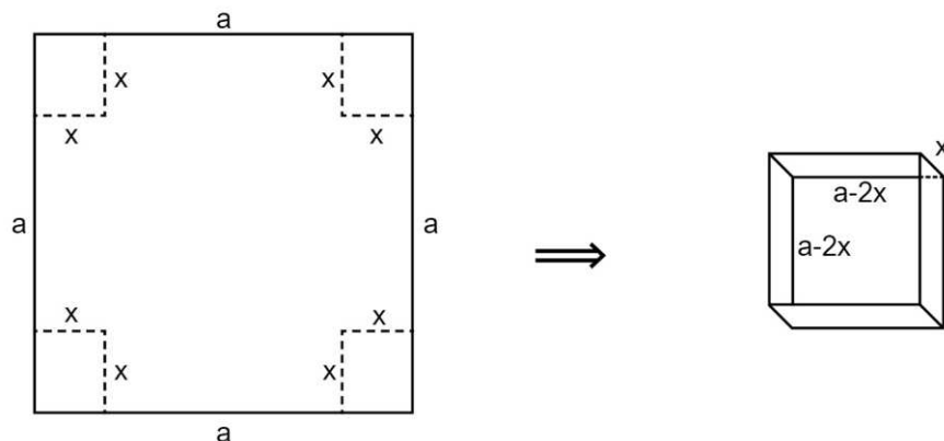
Fig. 16: Square of side a .
