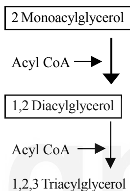
Figure 7.7 : Triacylglycerol synthesis
