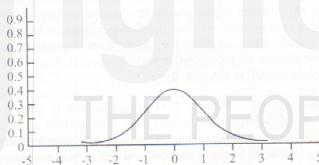
Figure 1.5: The standard normal distribution
