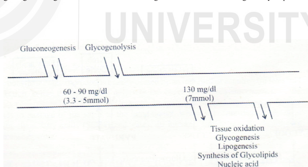
Figure 3.4: Regulation of blood glucose
