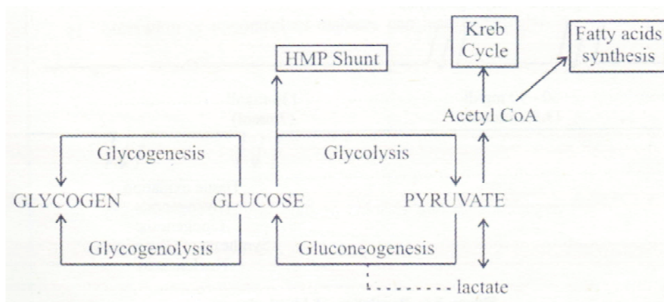
Figure 3.3: Integrated overview of metabolic pathways of carbohydrates
