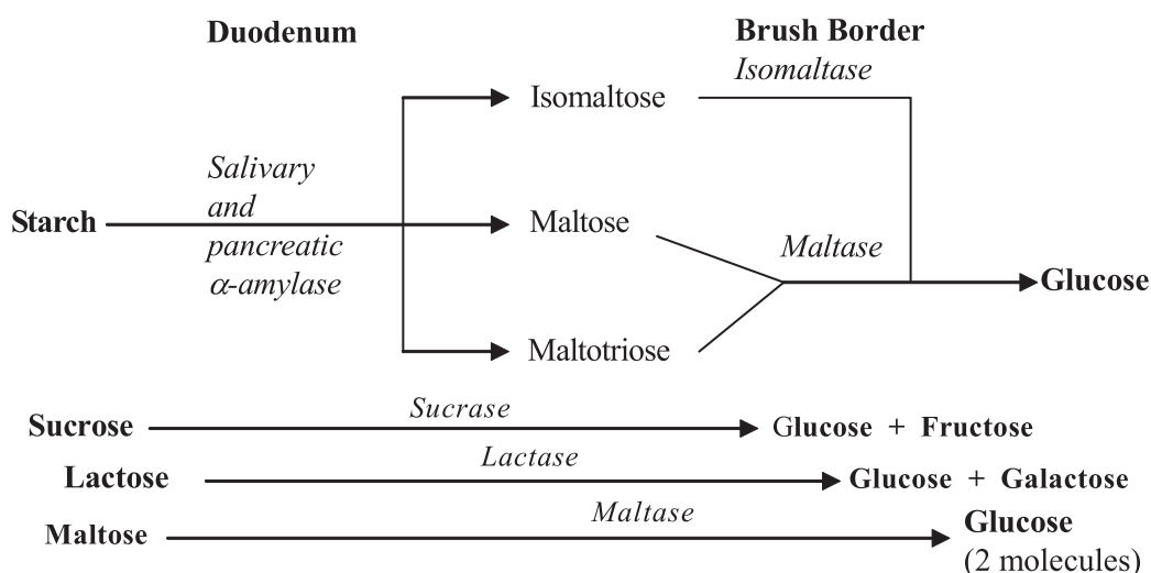
Figure 3.1: Digestion of carbohydrates
