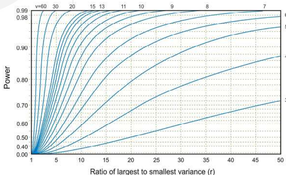
Figure 2.1: Power curve for \alpha = 0.1 and k = 4
