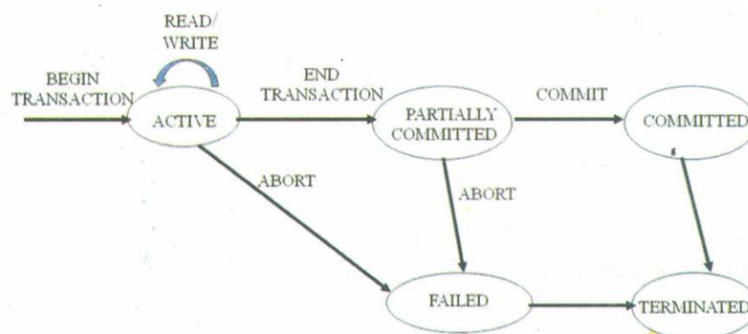
Fig. 2: Transaction states
