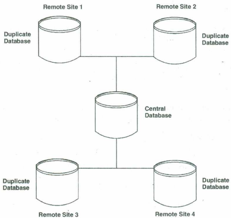
Fig. 2: Full Replicated Database
