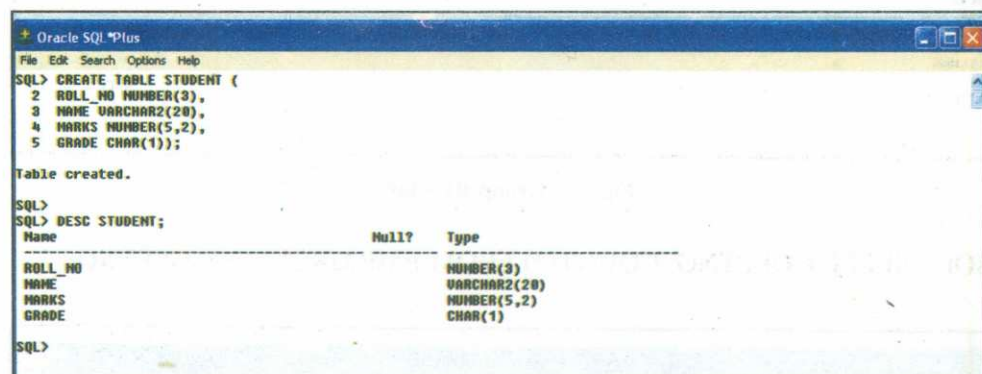
Fig. 34: Table created and described
