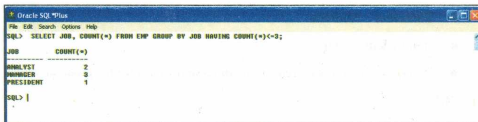
Fig. 33: Having Clause
