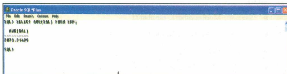
Fig. 29: Average function
