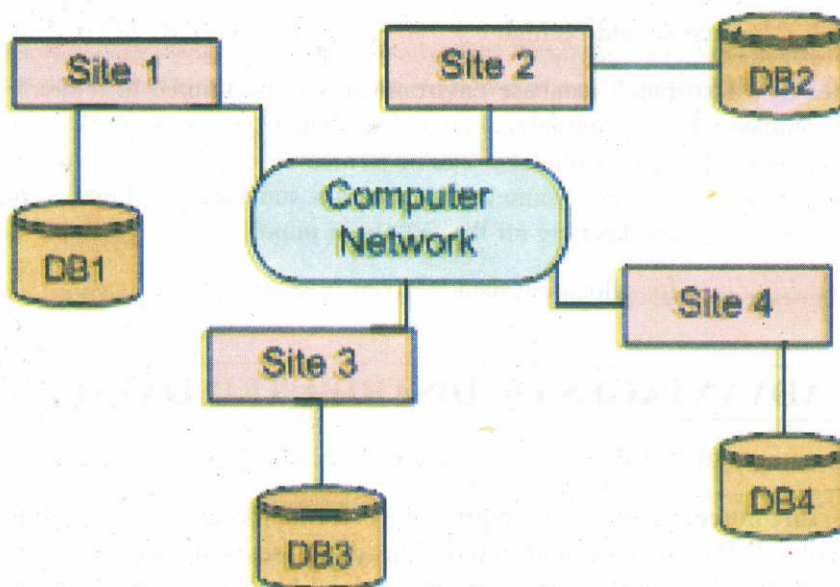
Fig. 1: Distributed Database
