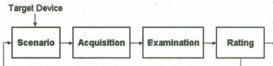
Fig. 1: Tool Assessment
