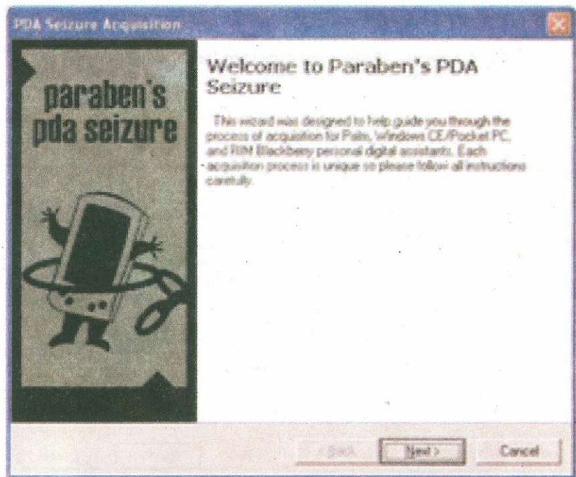
Fig. 7: Acquisition Wizard
