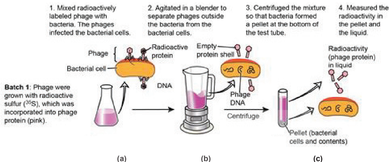
Fig. 2.2: The Hershey and Chase Experiment where phages were grown with radioactive S-35.
