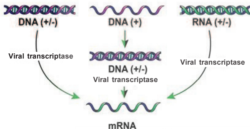
Fig. 1.18: Mechanism of action of viral transcriptase.
