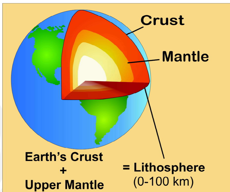
Fig. 2.3: The Lithosphere.
