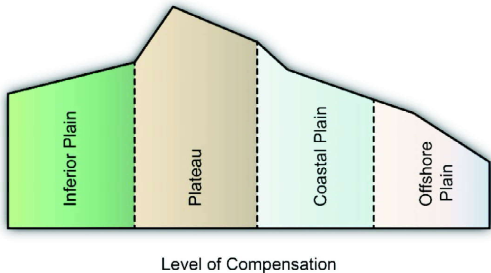
Fig. 4.7: Level of Compensation according to Hayford.
