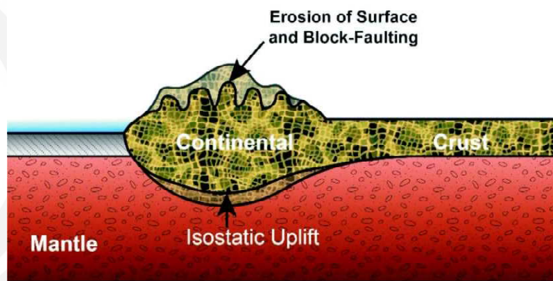
(b) End of the Orogenic stage.
