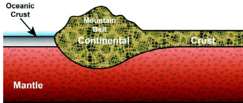
(a) Isostatic Uplift and Block-faulting stage.
