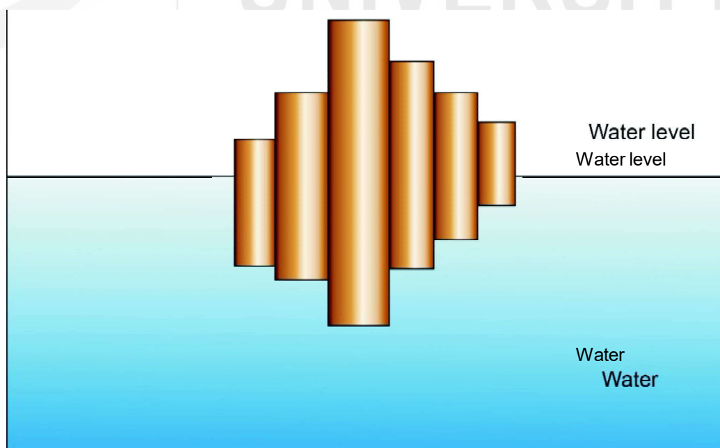
Fig. 4.4: Uniform density of different level features with varying thickness.
