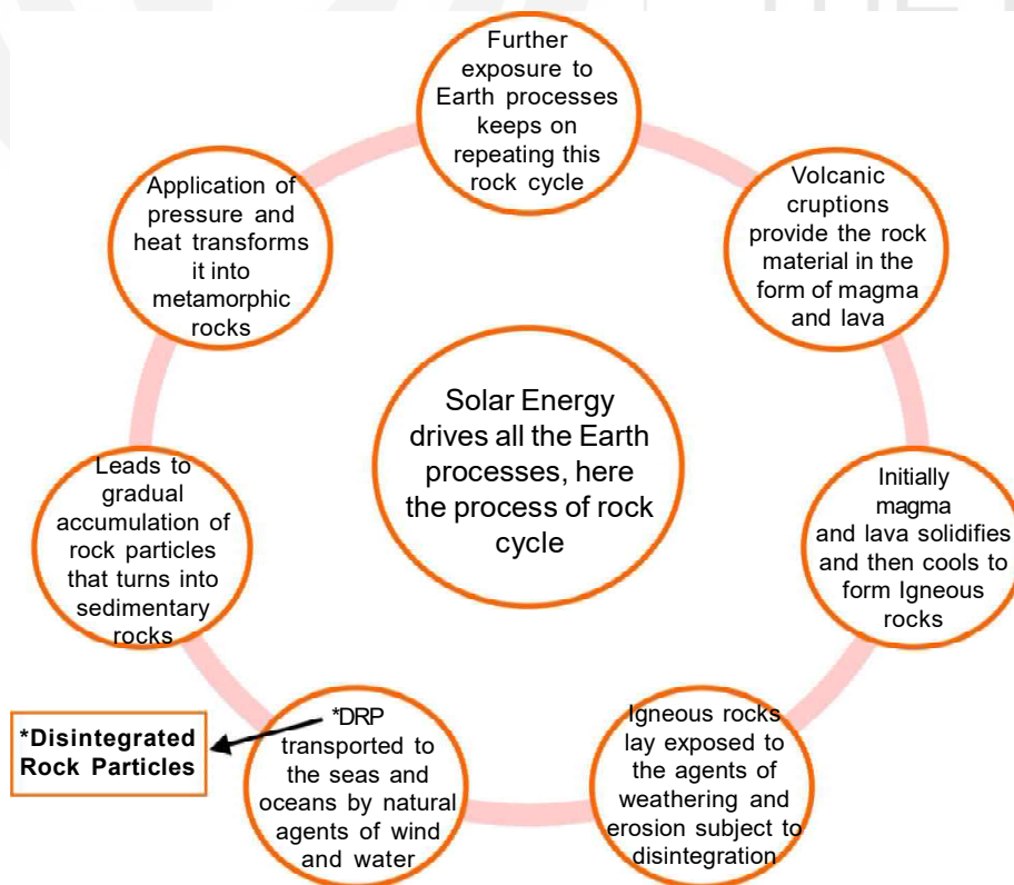
Fig. 3.1: Rock Cycle.
