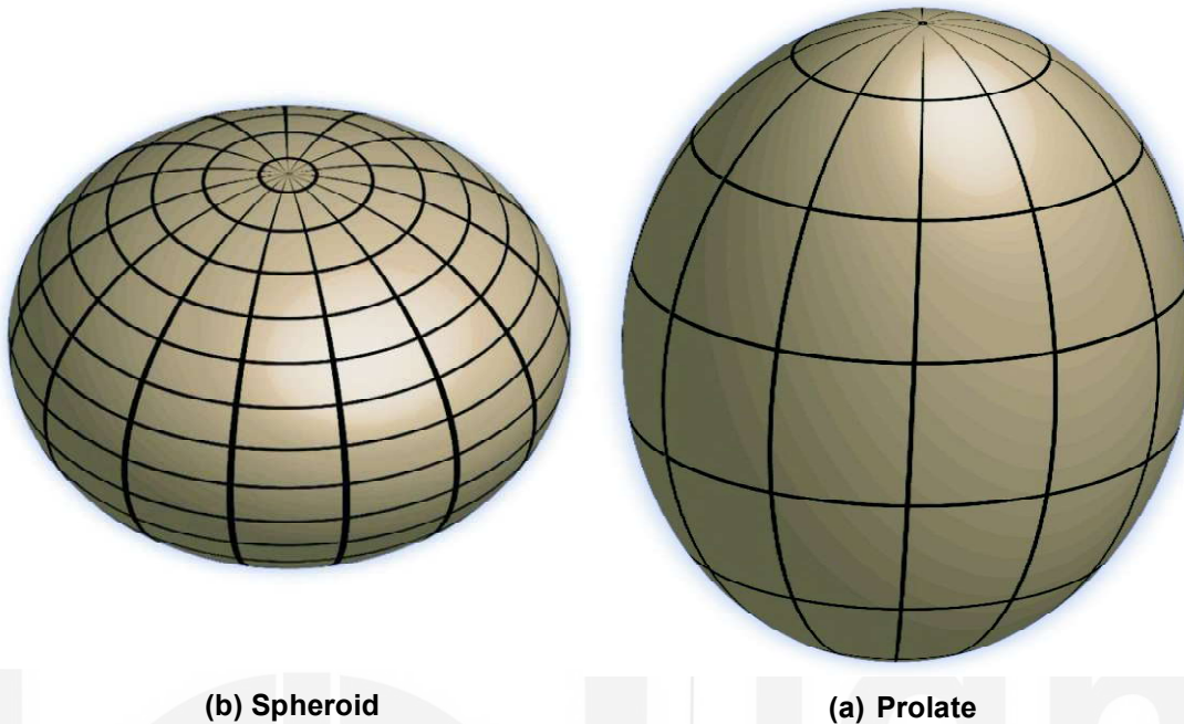
Fig. 4.1: Shape of the Earth (a) Prolate Spheroid; (b) Oblate Spheroid.
