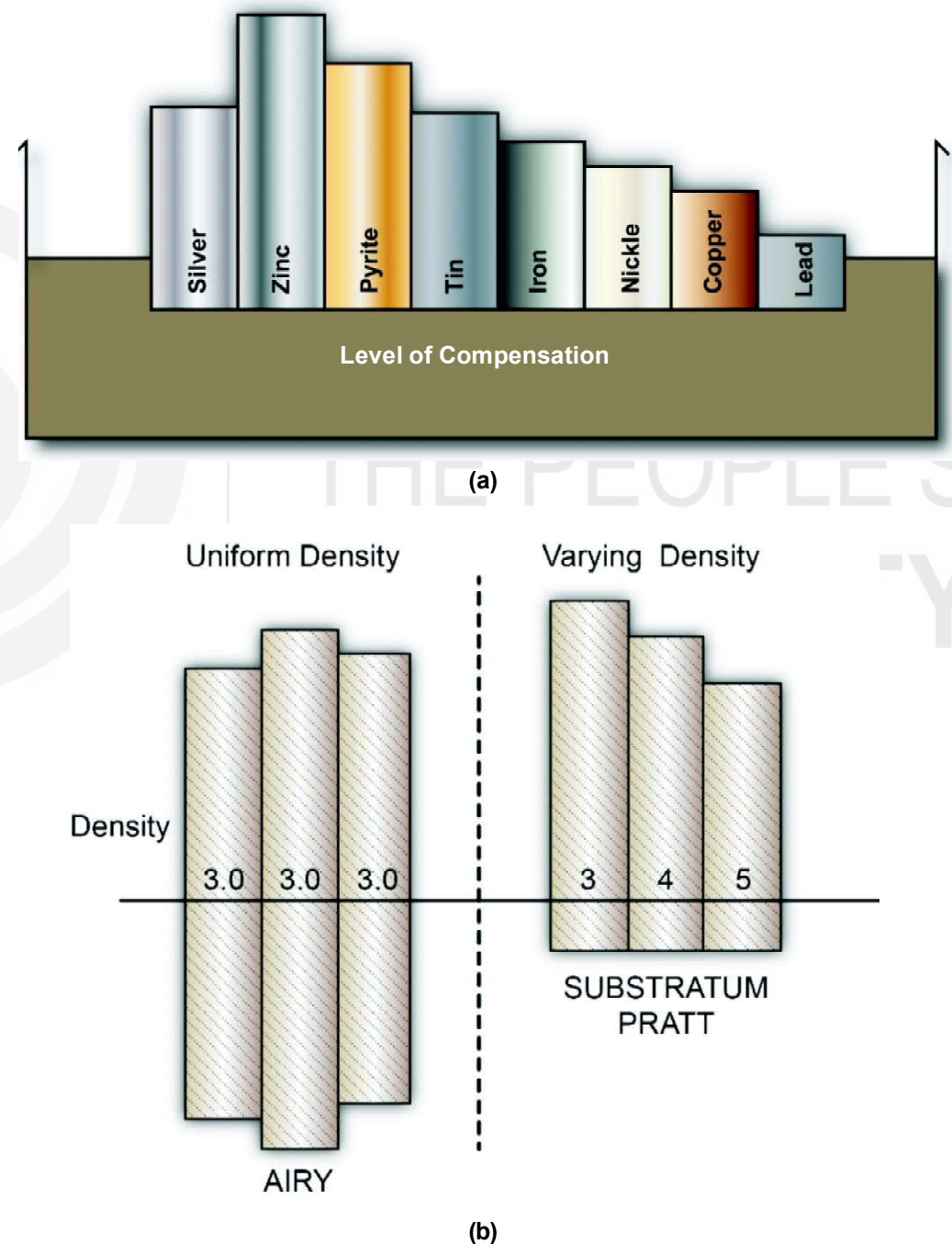
Fig. 4.6: a) Level of Compensation; b) Comparison between Airy and Pratt.
