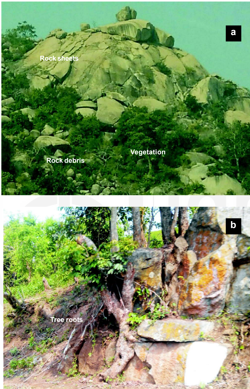
Fig. 8.3: a) Rock exfoliation; b) roots grow into rock cracks leading to formation of fractures.
