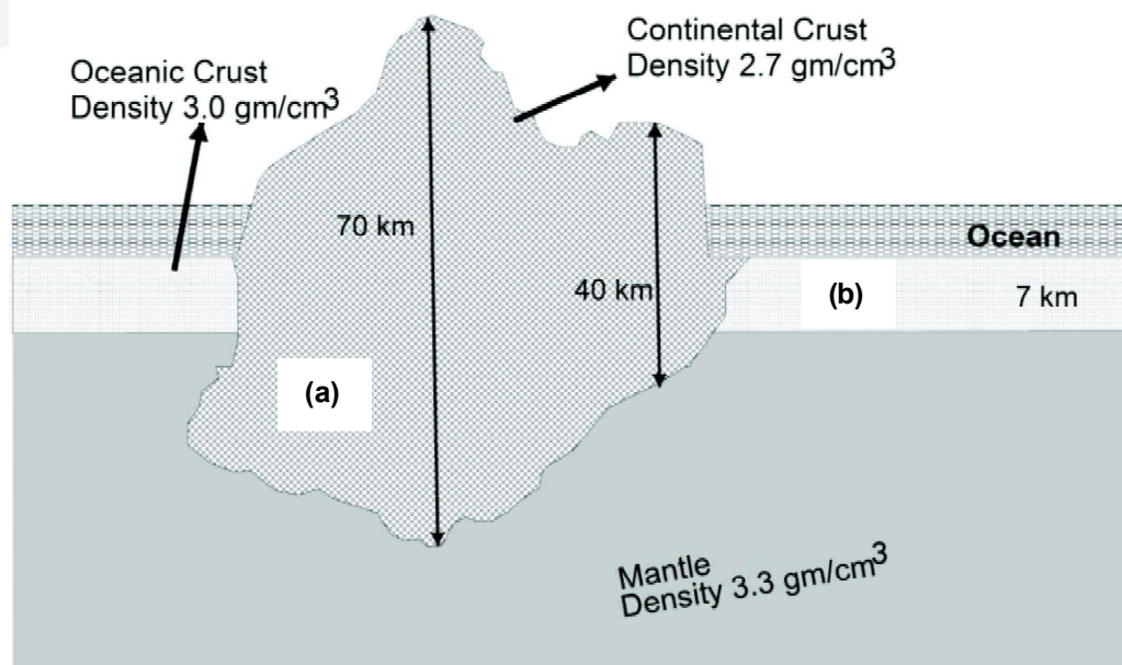
Fig. 7.2: Zones of the Earth's crust a) continents stand high due to continental crust which is thick and less in weight; b) oceans are low because oceanic crust is very thin and dense.
