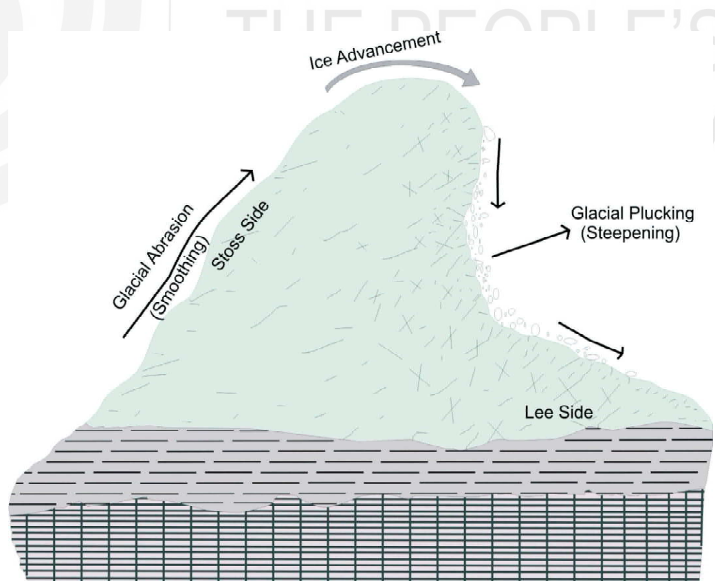
Fig. 9.3: Formation of roche moutonnee; this feature is produced by both mountain glaciers and continental ice sheets.
