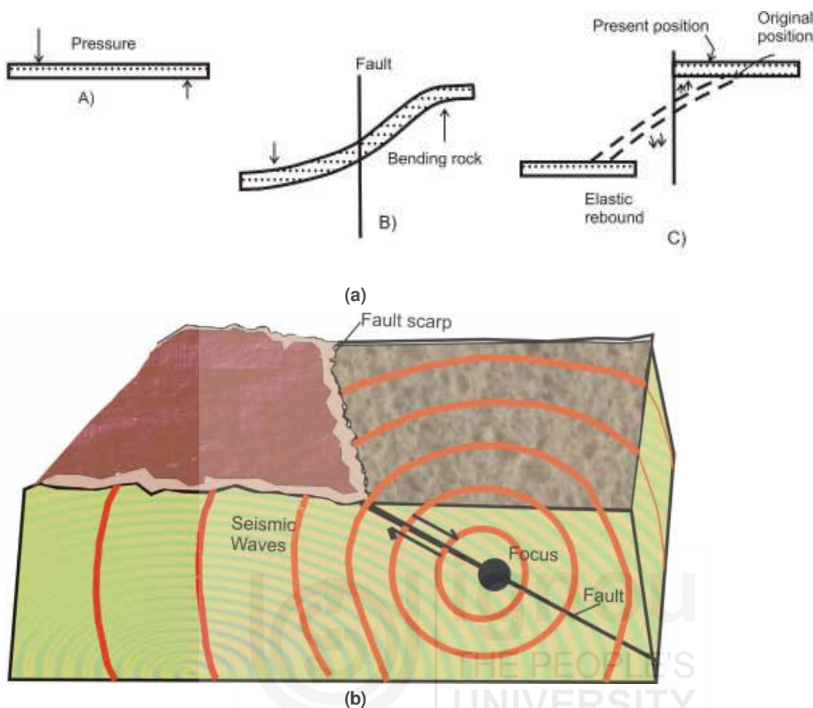
Fig. 4.2: a) Elastic rebound showing stages of rupture. A, B and C represent different stages of rupture; and b) Schematics showing generation of an earthquake. Earthquakes are usually associated with slippage along a fault.
