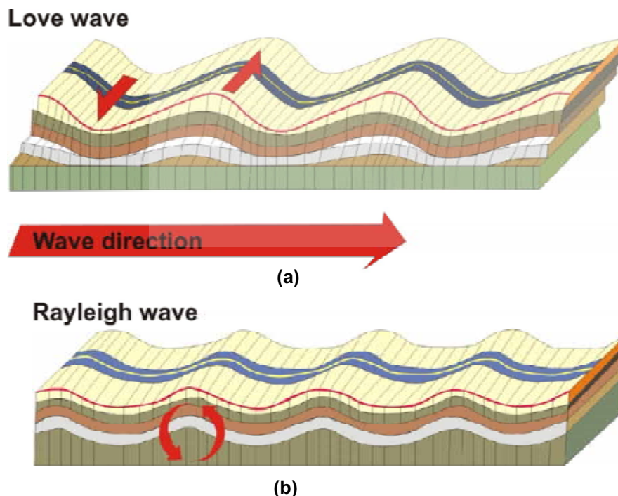
Fig. 3.4: Diagram showing Surface waves moving on the Earth's surface: Love wave in top panel and Rayleigh wave in bottom panel.
