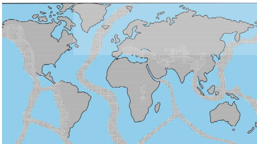
Fig. 4.6: Distribution of earthquakes: the shaded areas are the zones of active epicenters.
