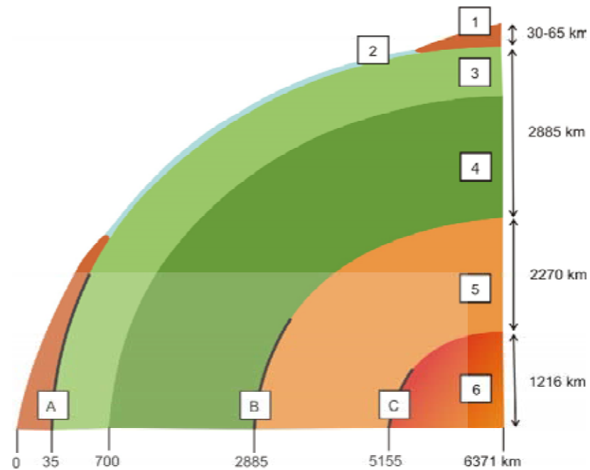
Fig. 3.8: Schematic section of the interior of the Earth: 1. continental crust, 2. oceanic crust, 3. upper mantle, 4. lower mantle, 5. outer core, 6. inner core. A: Mohorovicic discontinuity, B: Gutenberg Discontinuity, and C: Lehmann-Bullen discontinuity. Note that there is another discontinuity i.e. Conrad discontinuity, which is between upper and lower crust.
