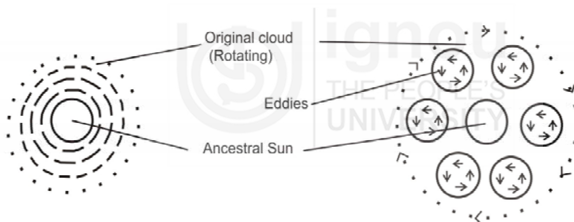
Fig. 2.3: Schematics showing process of condensation.
