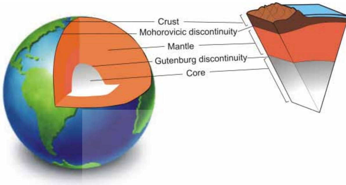
Fig. 3.6: Layered structure of the Earth.
