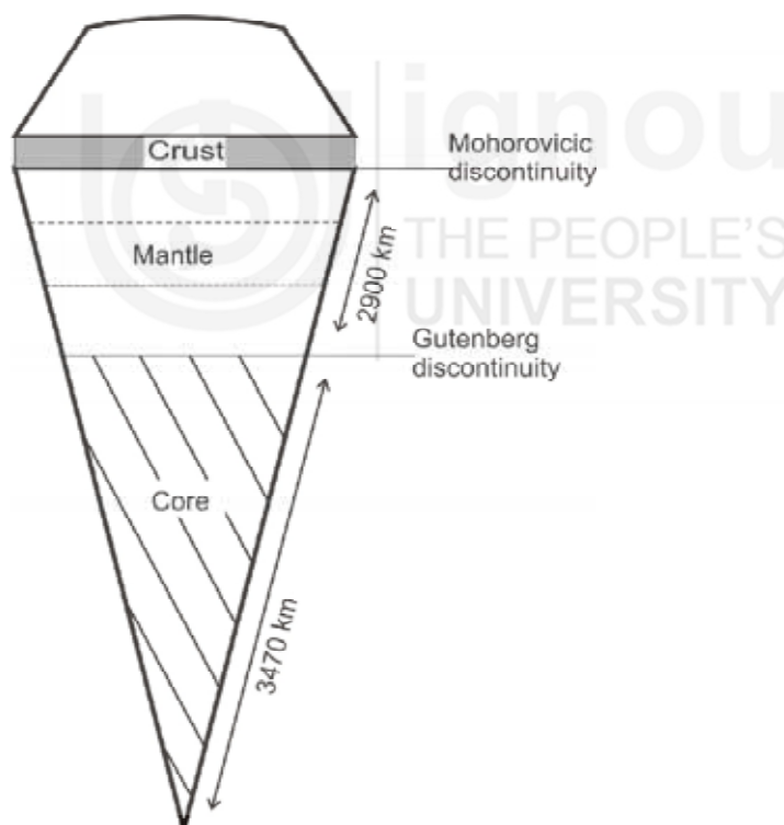
Fig. 2.4: Wedge of the Earth showing the crust, mantle and core with major boundaries.
