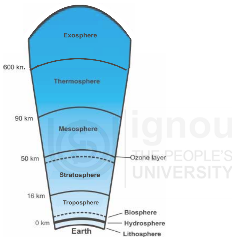
Fig. 3.1: Layers of atmosphere.
