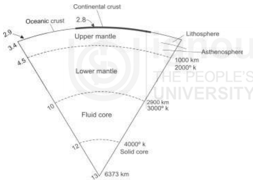
Fig. 3.7: Cross section of Earth showing the crust, mantle and core with major boundaries. Depths are in km from surface; temperature in degrees K; figures on left are mass density in 10^3 \text{ kg/m}^3 . (Source: After Bott, 1982)
