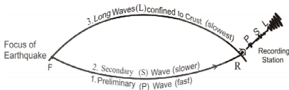
Fig. 4.3: Diagrammatic representation of earthquake waves – its origin, movement and the recording station.
