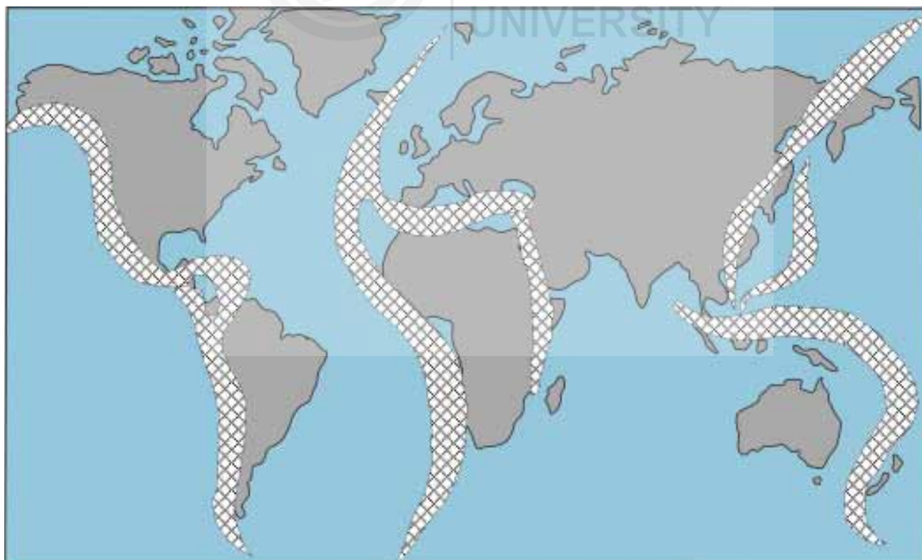
Fig. 4.15: Distribution of volcanic belts in world map.
