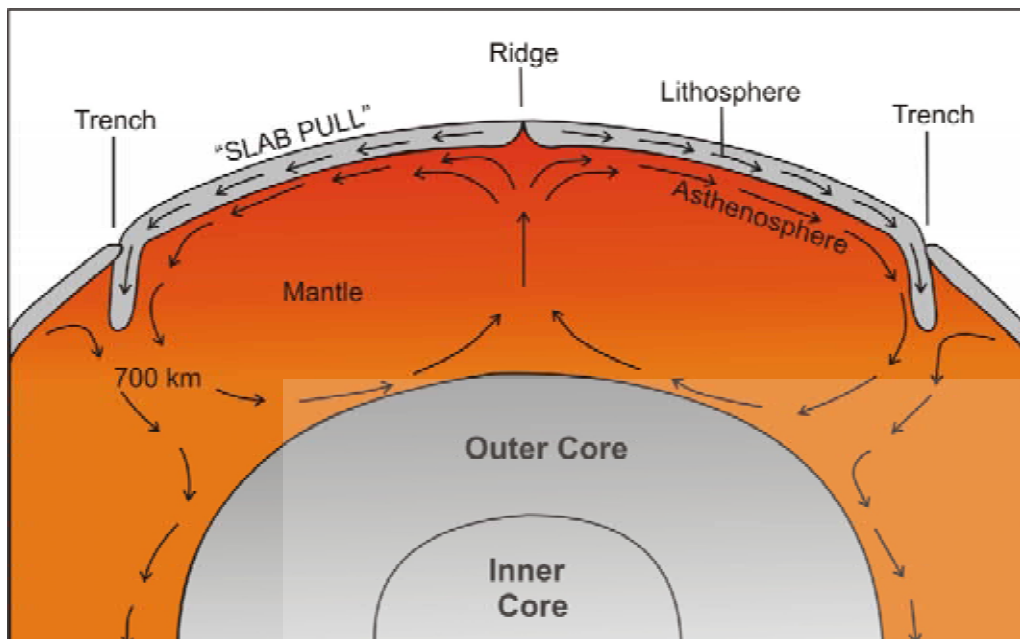
Fig. 16.7: Cells of convection currents in the interior of the Earth.
