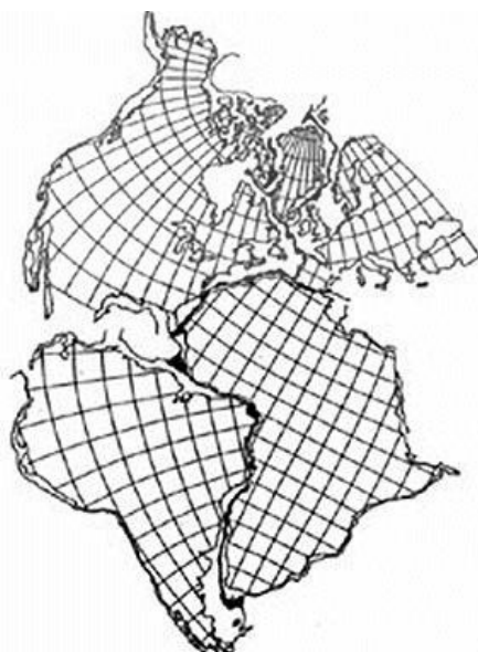
Fig. 15.1: Jigsaw fit of the coastlines of Atlantic Ocean. (Source: http://www.age-of-the-sage.org/plate_tectonics/continental_drift.html )
