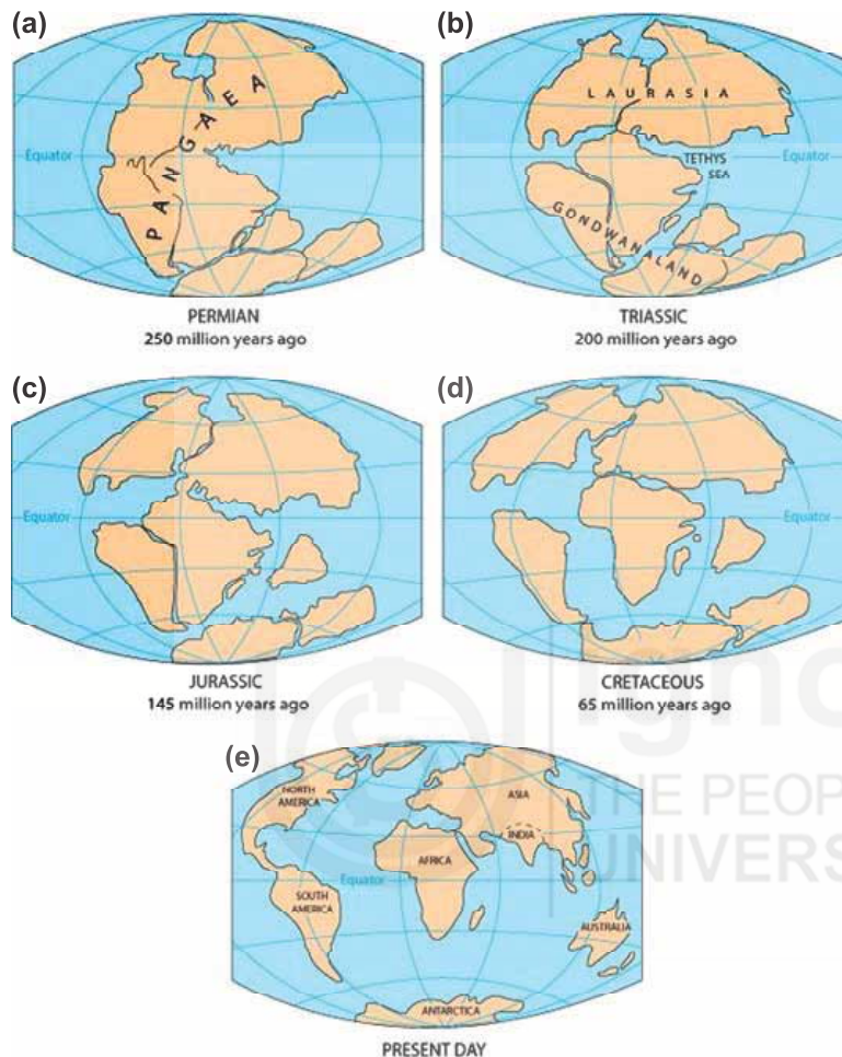
Fig. 16.13: Stages of Evolution of Himalaya from Permian period onwards. (Source: http://i.livescience.com/images/i/000/047/334/i02/Pangaea.jpg?1365037770 )
