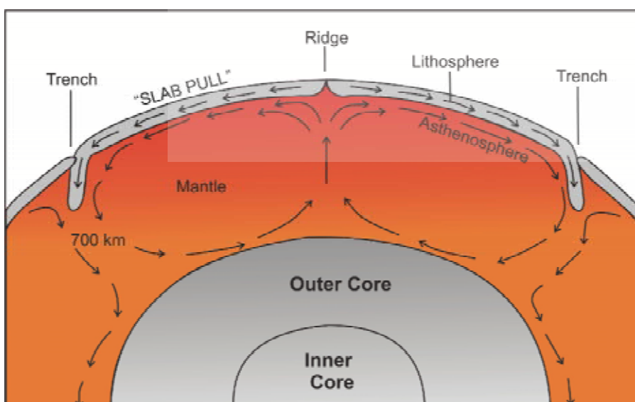
Fig. 15.7: Cells of convection currents in the interior of the Earth.
