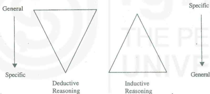
Fig. 3.1 : Deductive and inductive reasoning
