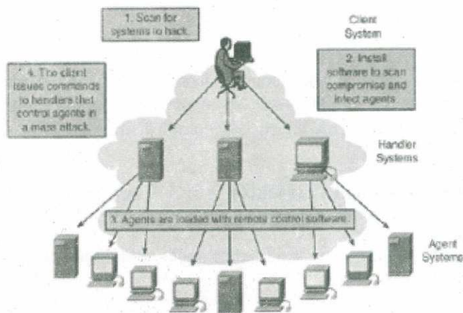
Fig. 14: DDoS Attack
