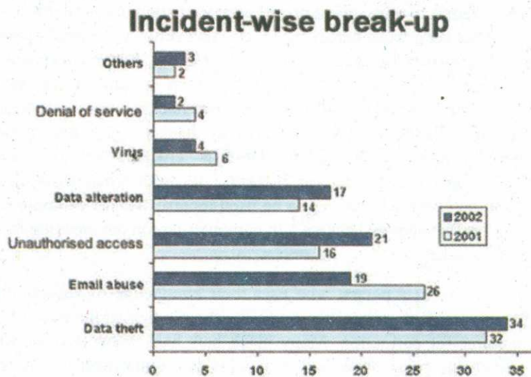
Fig. 1: Incident-wise break-up
