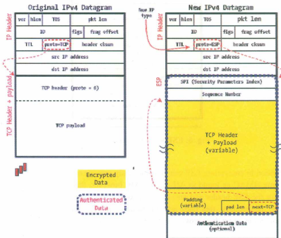
Fig. 7: IPsec in ESP Transport Mode
