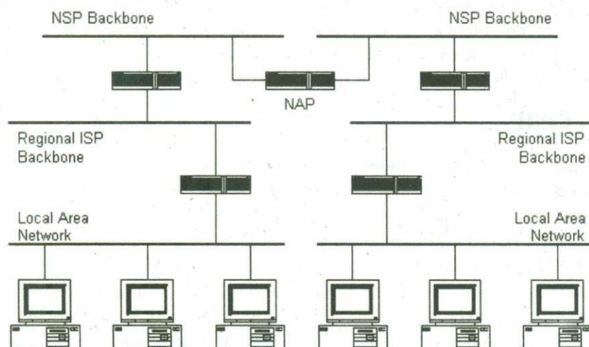
Fig. 7: Internet Architecture
