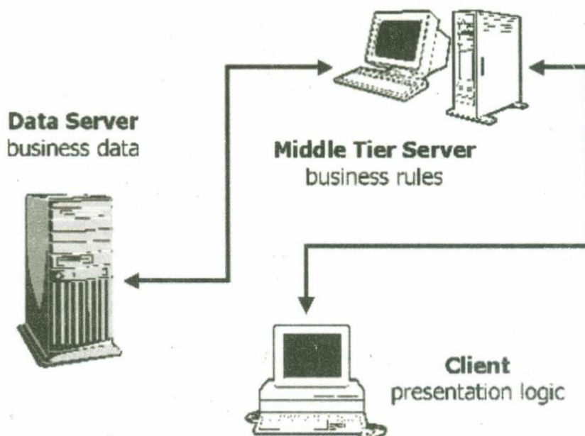
Fig. 3: Three-Tier Architecture
