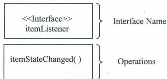
Fig. 14: Icon Used in UML to Represent Interface
