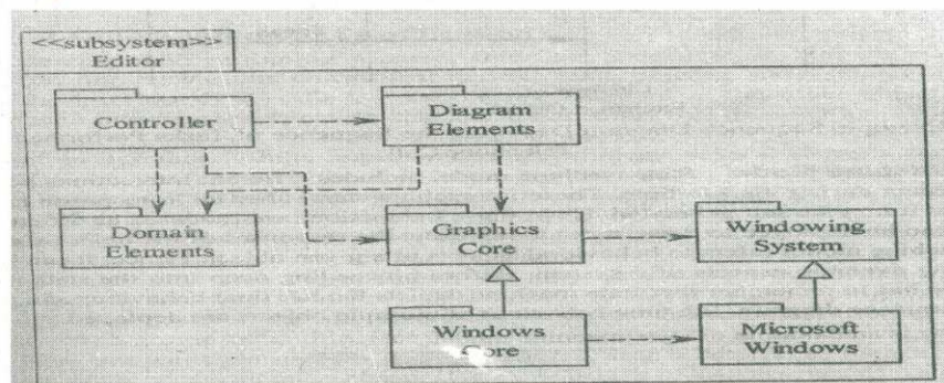
Fig. 11: Example figure Depicting the Subsystem Modeling
