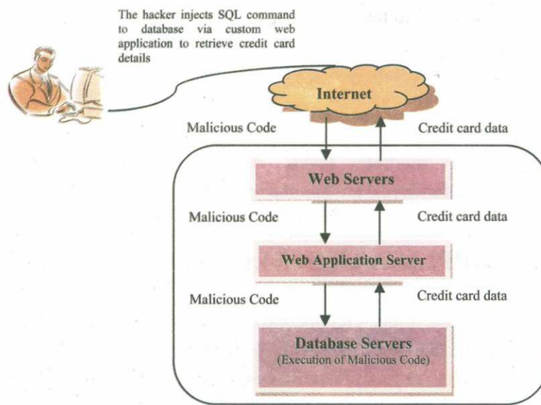
Fig. 2: SQL Injection
